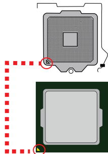
Figure 2-6 CPU installation
