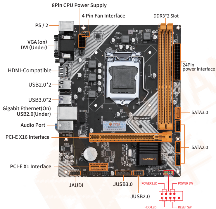
1-1 B75 Motherboard Illustration
