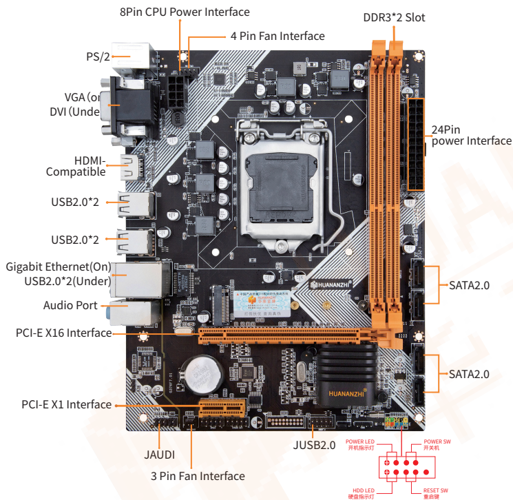
1-1 H61 MotherBoard Illustration
