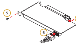
2-9 Graphics Card Installation
