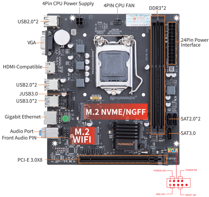
1-1 H810M-VH Motherboard Illustration
