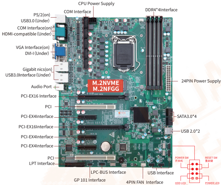
1-1 Q170 Motherboard Illustration
