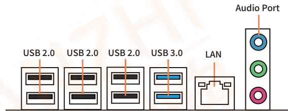
1-2 Overall Rear I/O Panel Display
