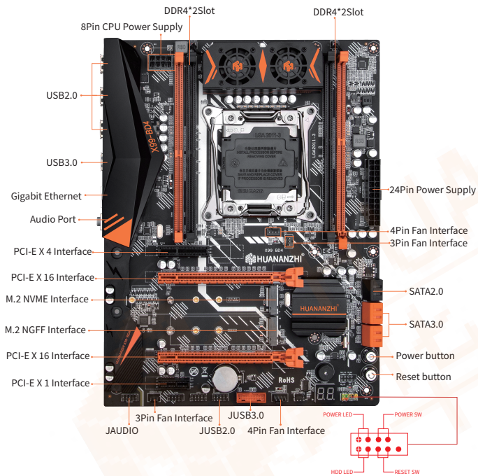
1-1 X99-BD4 Motherboard Illustration
