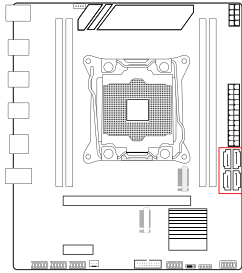
2-11 SATA Interface
