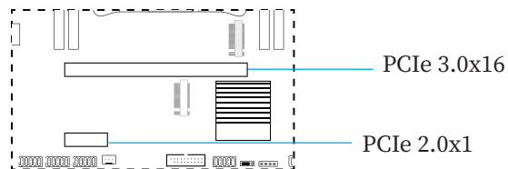
2-4 PCI Expansion Slot
