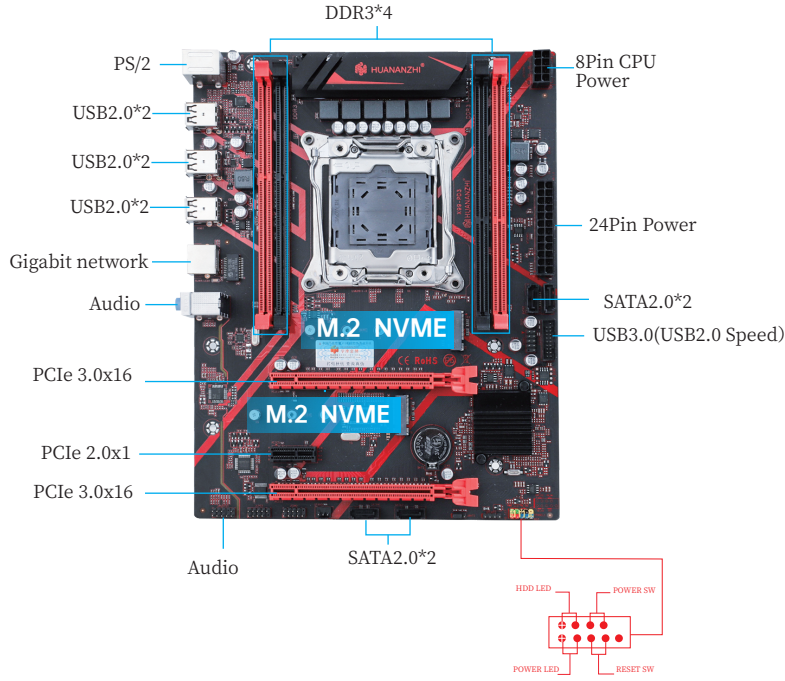
1-1 X99-PD3 Motherboard Illustration
