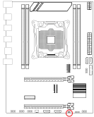
2-1 Clear CMOS Jumper CLR-CMOS
