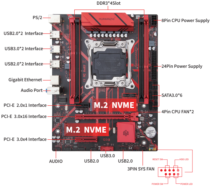
1-1 X99-QD3 Motherboard Illustration
