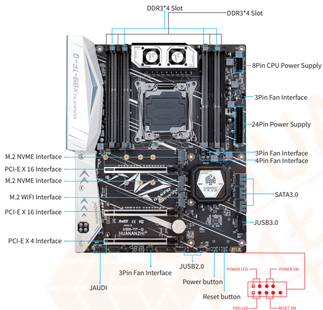
1-1 X99-TF-Q Motherboard Illustration
